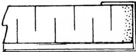
Panel 1" - 96 to 112 kg / m 3 (6 to 7lb. / ft 3 ) + 1/8" high density fiberglass bonded to face
